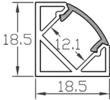
Technical Drawing
